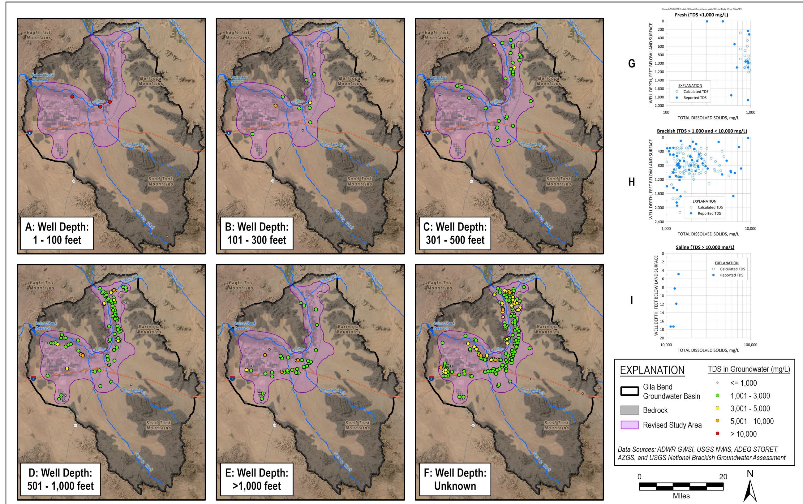
Figure 3-4. Gila Bend Groundwater Basin Water Quality
