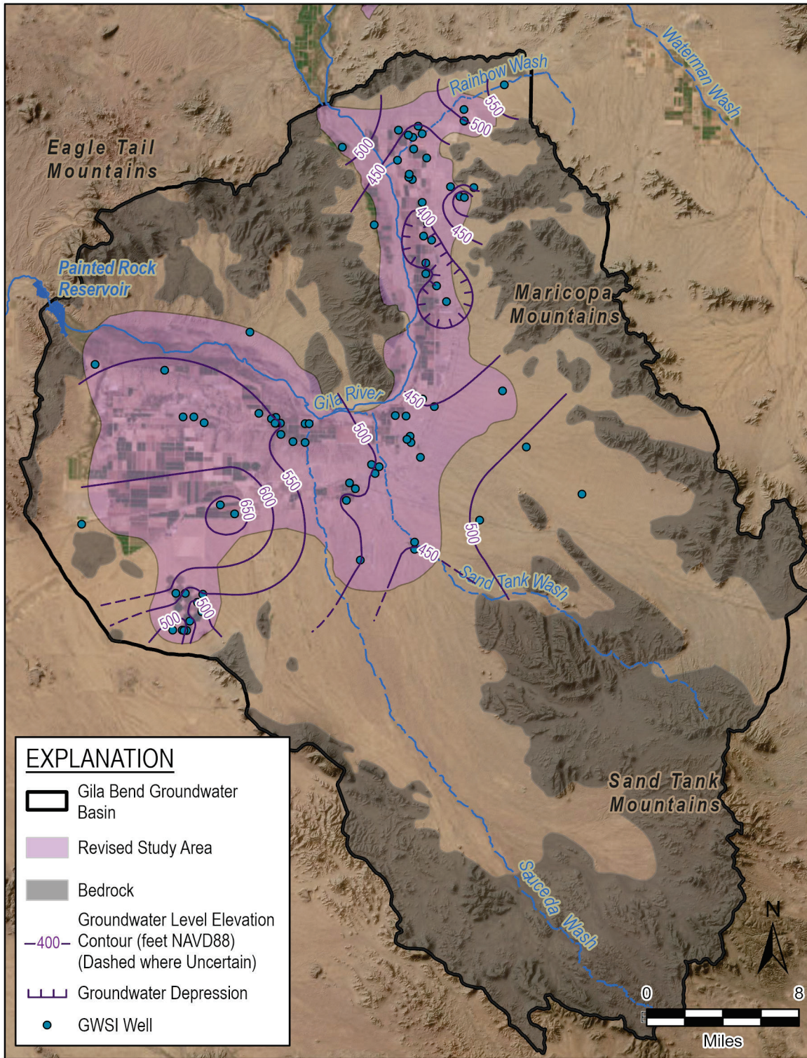
Figure 3-3. Gila Bend Groundwater Basin 2020 Groundwater Level Contours
