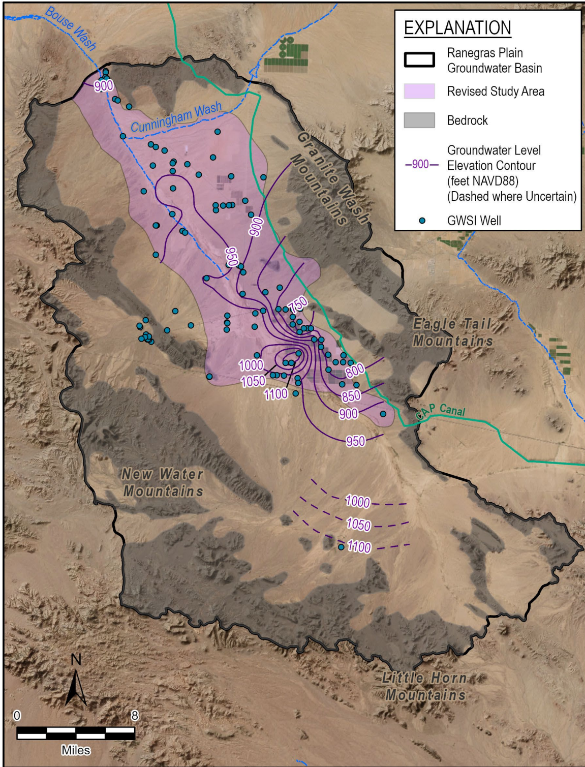
Figure 3-7. Ranegras Plain Groundwater Basin 2022 Groundwater Level Contours
