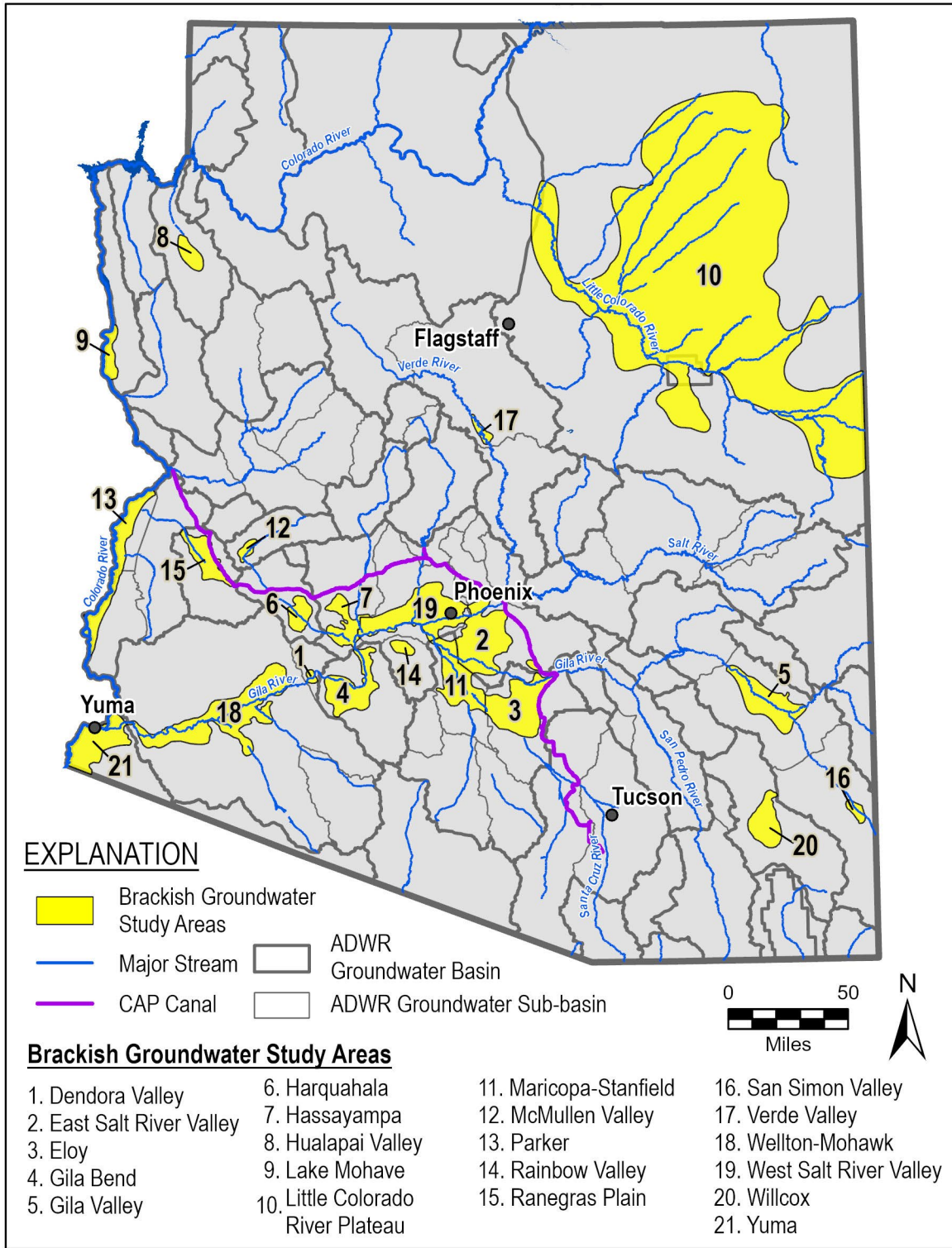
Figure 2-4. Initial Brackish Groundwater Study Areas
