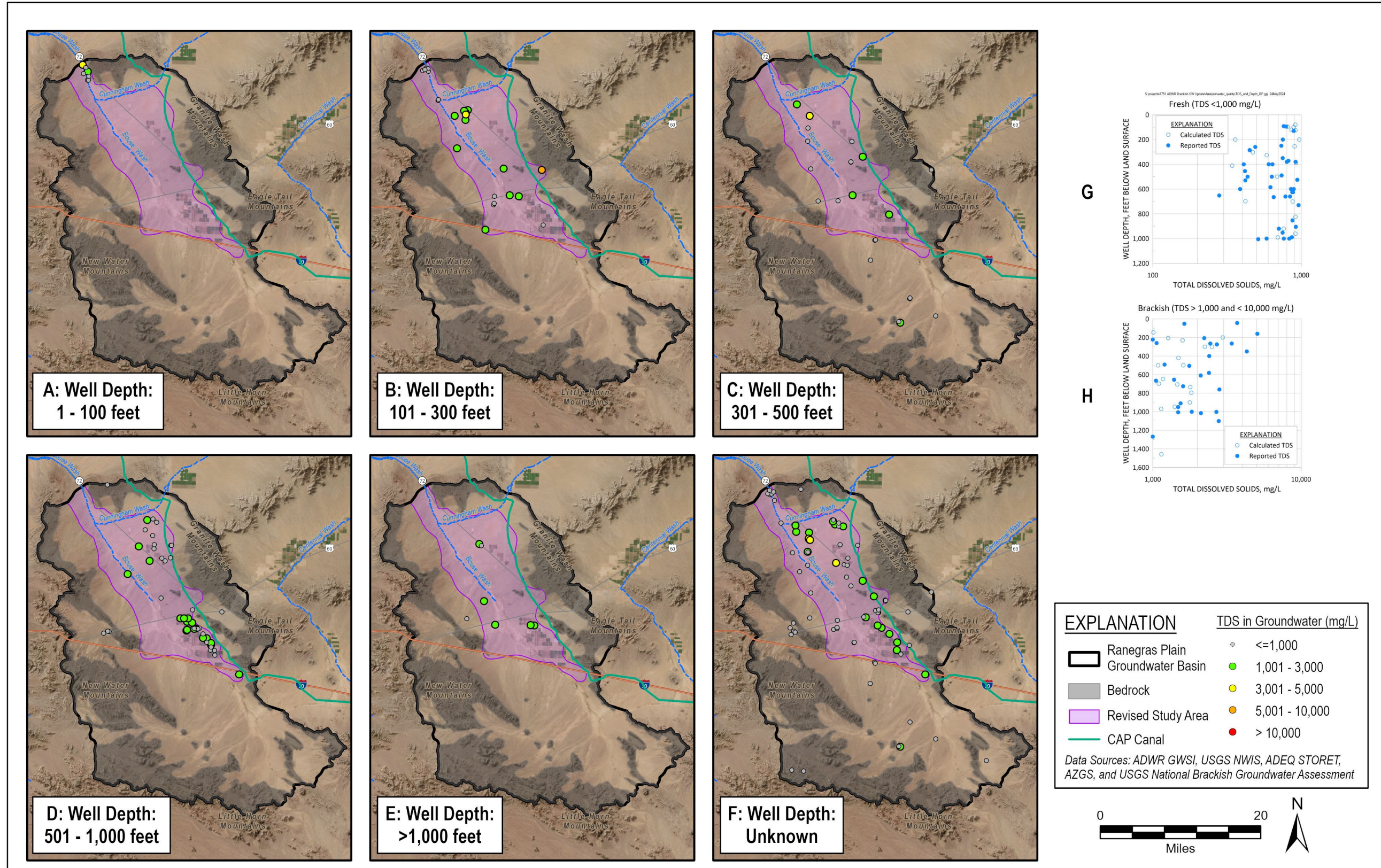
Figure 3-8. Ranegras Plain Groundwater Basin Water Quality
