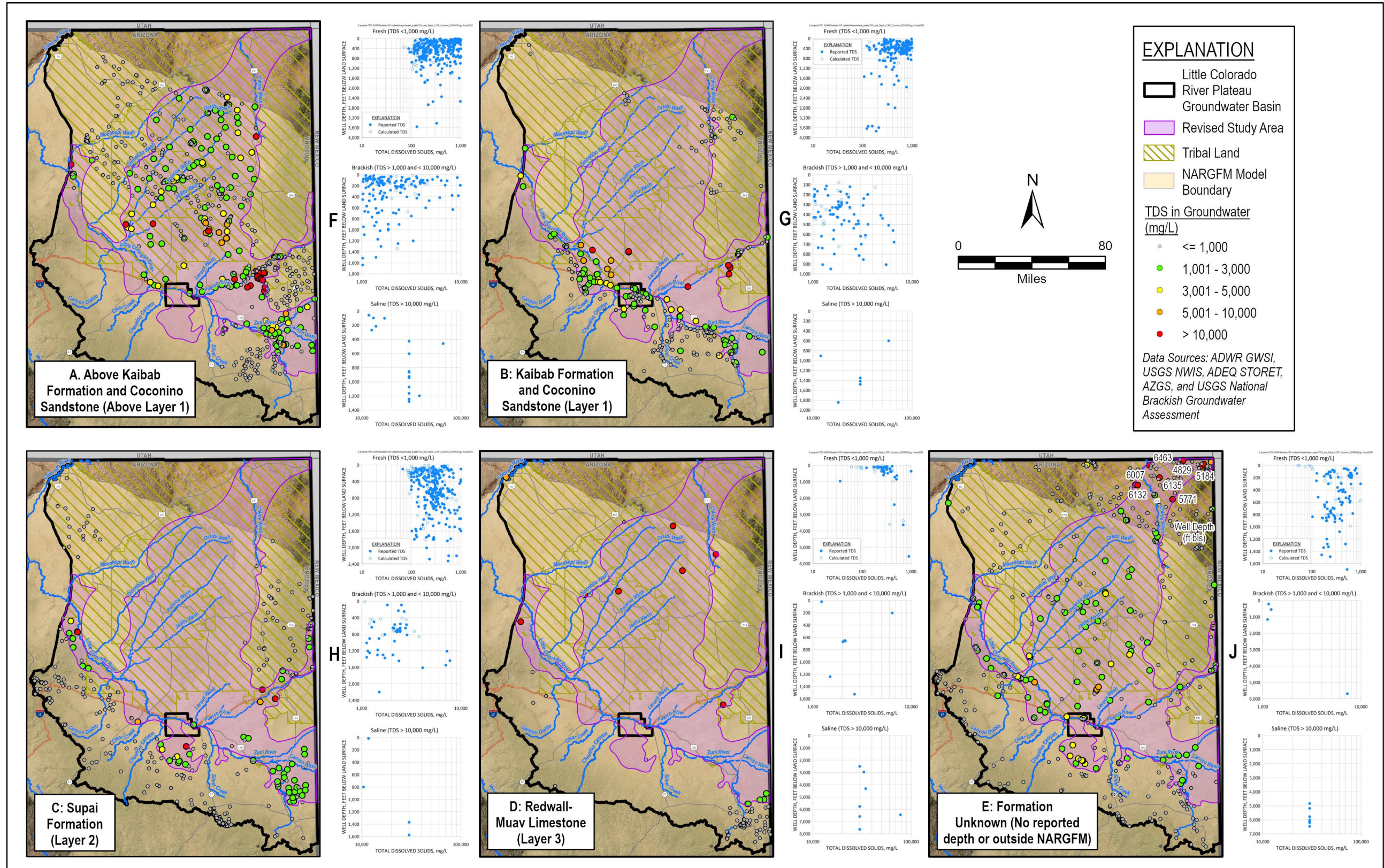
Figure 3-10. Little Colorado River Plateau Groundwater Basin Water Quality
