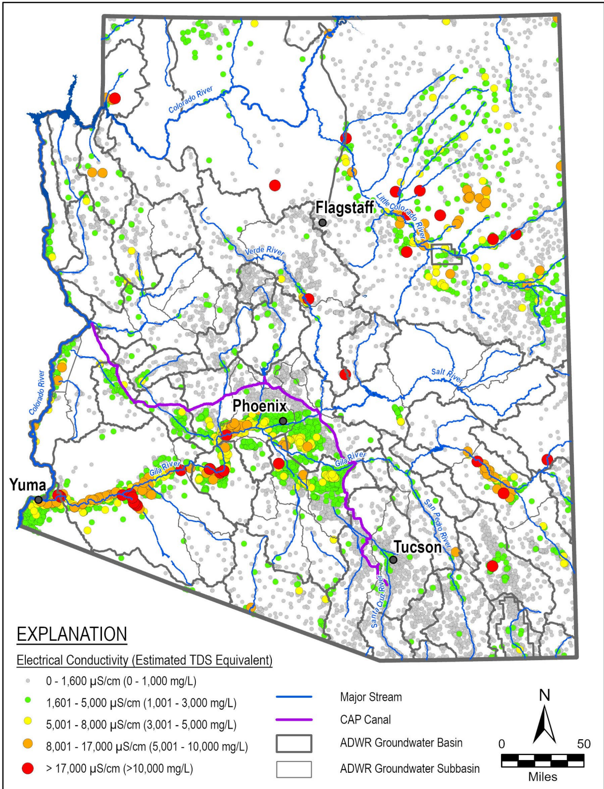
Figure 2-1. Most Recent EC Data from NWIS and GWSI
