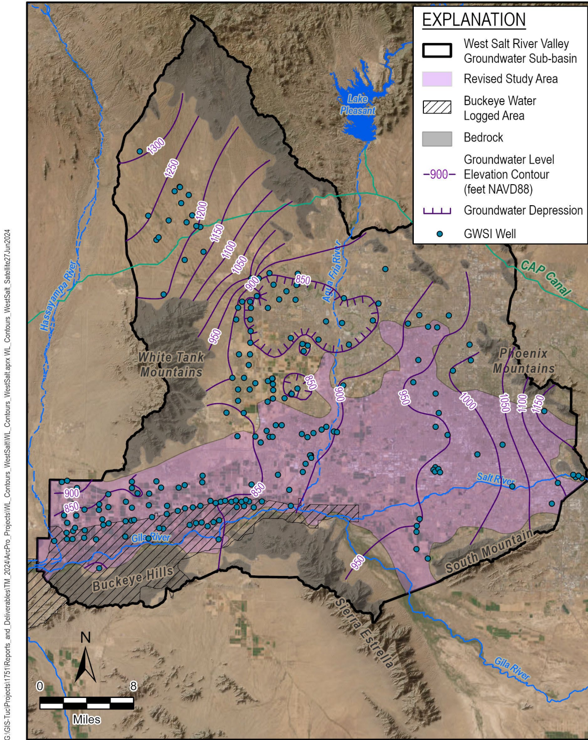
Figure 3-5. West Salt River Valley Groundwater Sub-Basin 2023 Groundwater Level Contours
