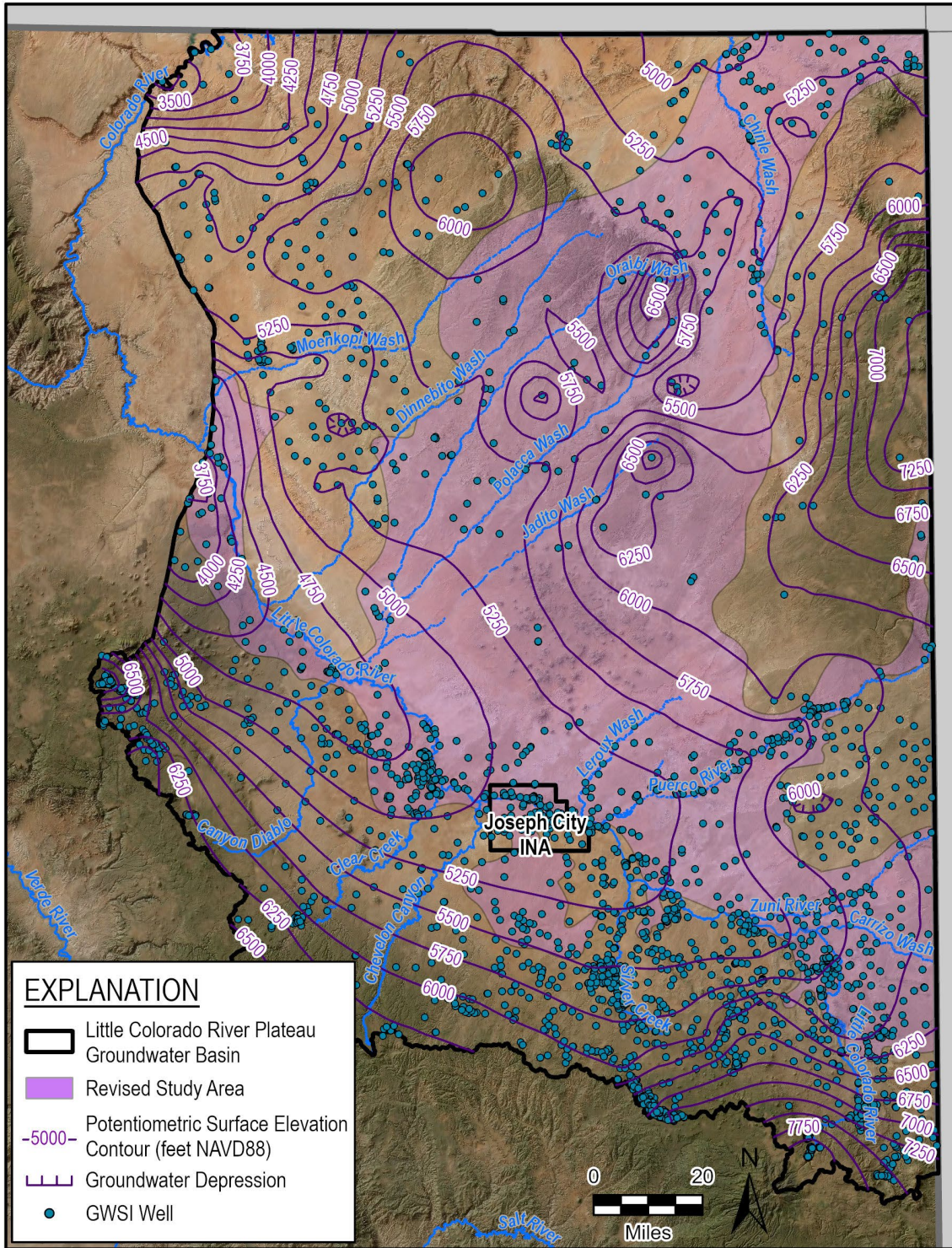
Figure 3-9. Little Colorado River Plateau Groundwater Basin 2022 Groundwater Level Contours
