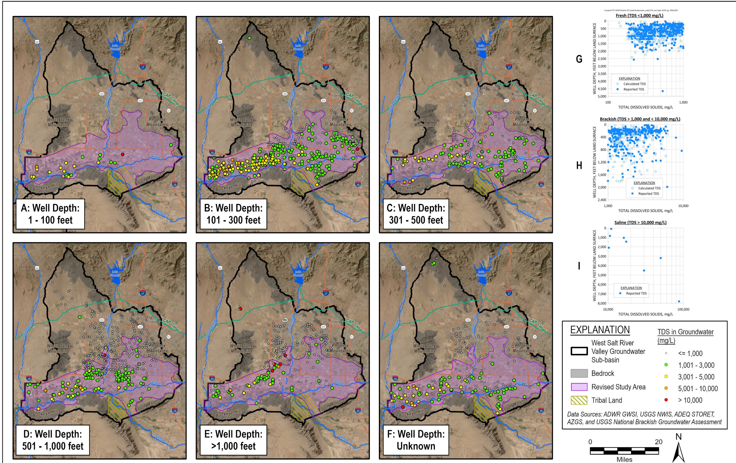
Figure 3-6. West Salt River Valley Groundwater Sub-Basin Water Quality
