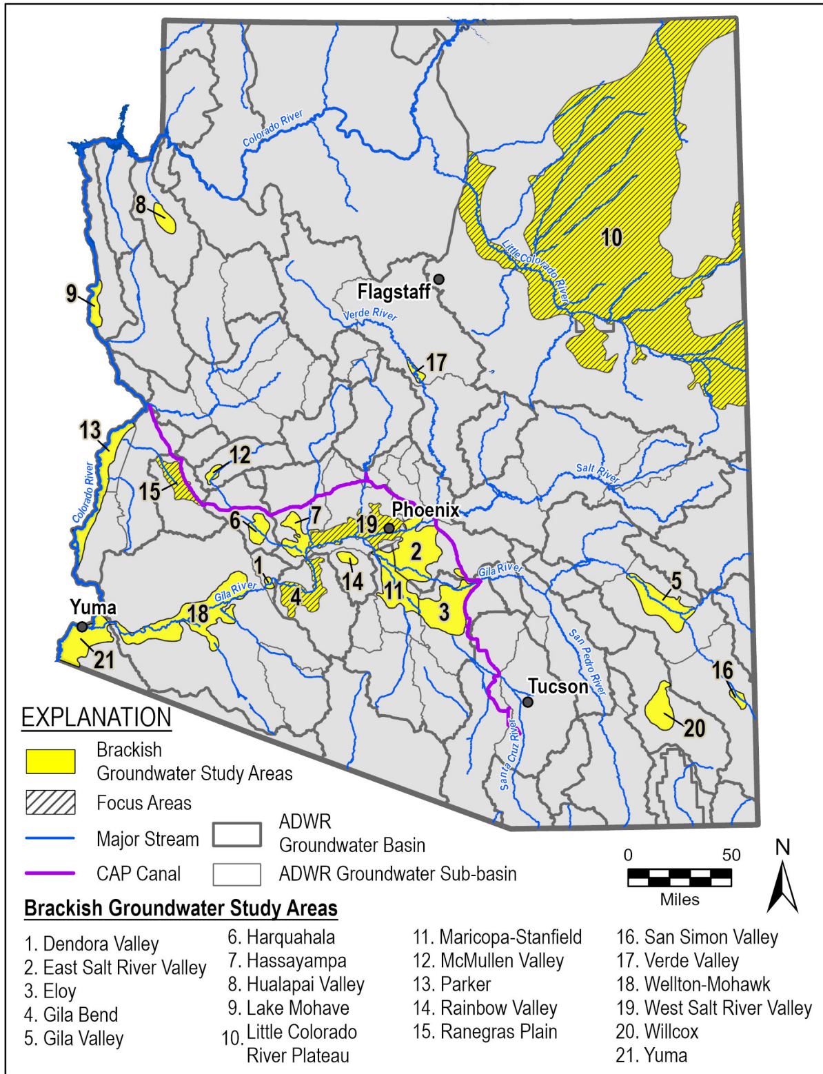
Figure 3-1. Refined Brackish Groundwater Study Areas
